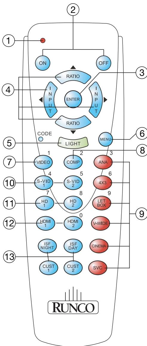
Figure 2-6. DHD Controller/VX-44d/-55d Remote Control
